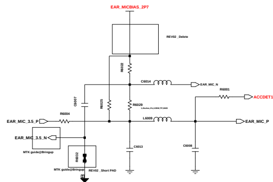
EAR MIC
