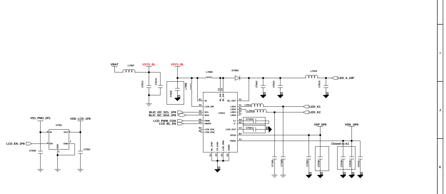
CAMERA MIPI SWITCH LCD_LDO BLIC Engineer: CAMERA, DISPLAY Drawn by: R&D CHK: TITLE: Size: DOC CTRL CHK: SM-A02 MFG ENGR CHK: Changed by: Date Changed: Time Changed: QA CHK: REV: Drawing Number: Page: 7/7 2 3 4 5 6 7 8 9 10 11 12 13 14 15 16
